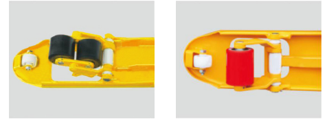
Option of single and tandem fork rollers
